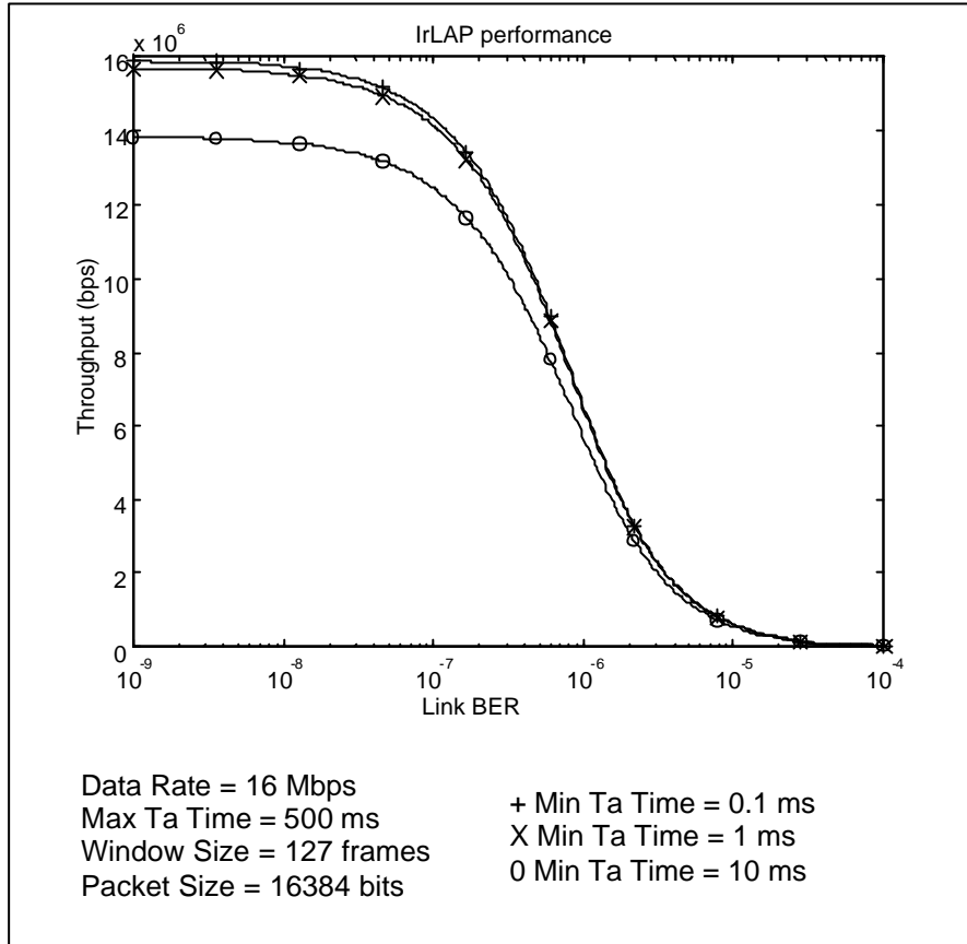
Figure 9: throughput Vs BER for 16 Mbps
