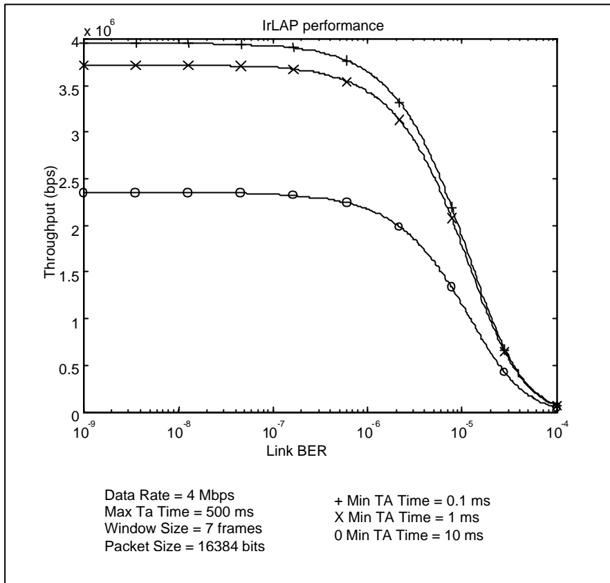
Figure 7: throughput Vs BER for 4 Mbps
