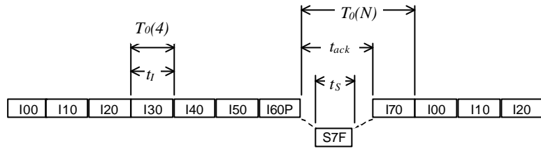
a) Error free transmission at w = 3 and w = N
