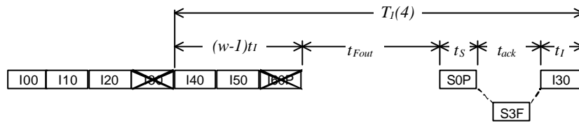
c) Retransmitted frames and F-timer delay due frame error at w = 4 and w = 1
