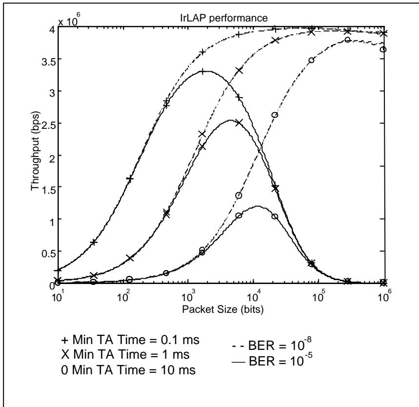
Figure 8: throughput Vs packet data size for 4 Mbps
