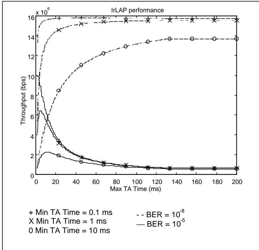
Figure 10: throughput Vs maximum turn-around time for 16 Mbps
