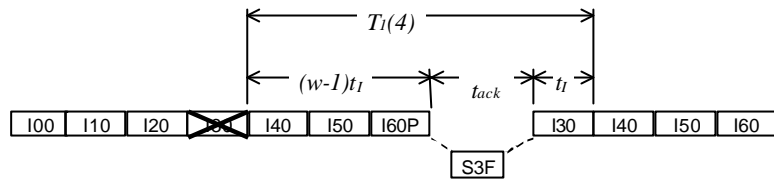
b) Retransmitted frames due to error frame at w = 4
