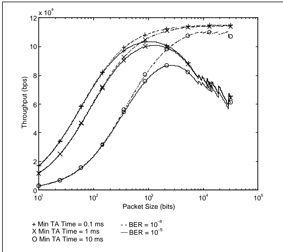
Figure 6: throughput Vs packet data size for 115200 bps
