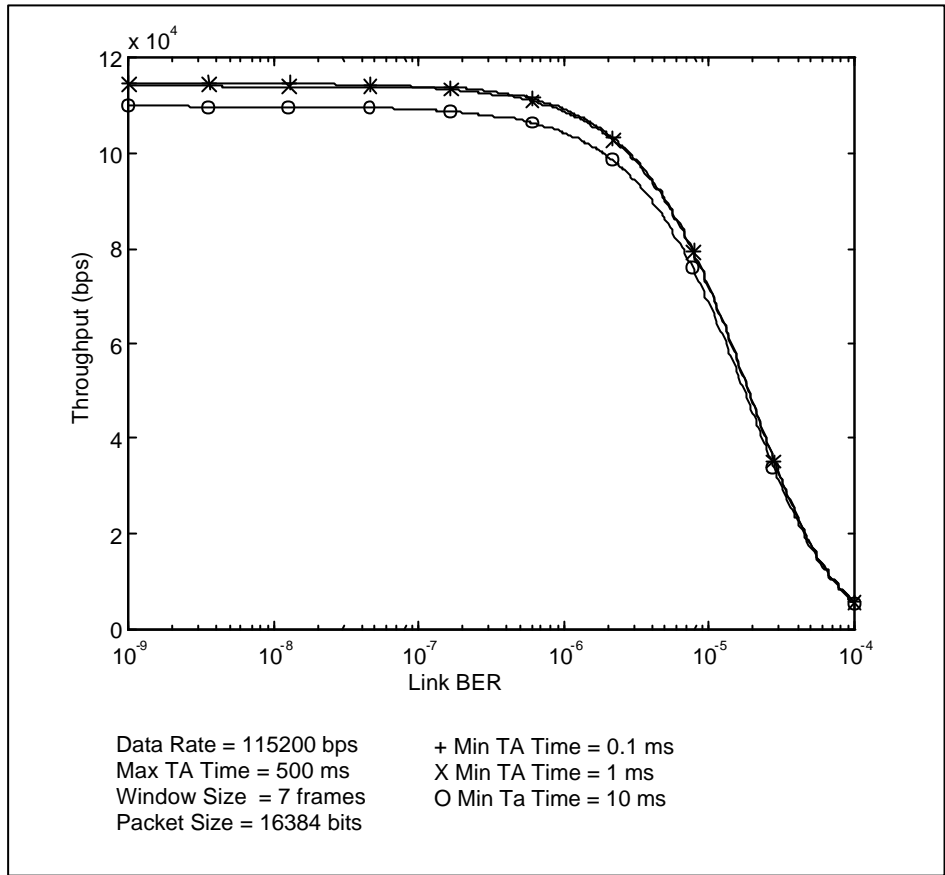
Figure 5 : throughput Vs BER for 115200 bps
