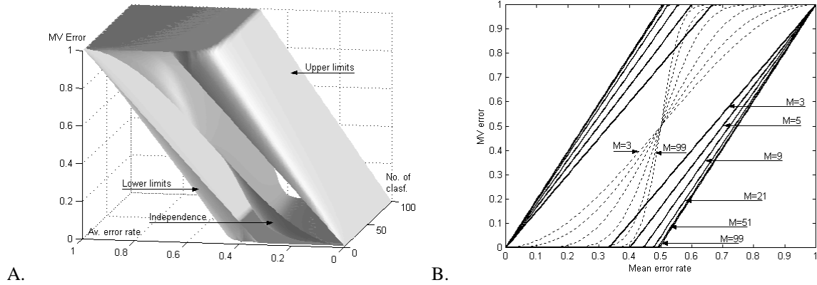
FIGURE 9. Majority voting error limits shown as a function of the number of classifiers and the mean classifier error. A. 3D plot including surface corresponding to MV errors for independent classifiers. B. 2D projections for the selected numbers of classifiers.
