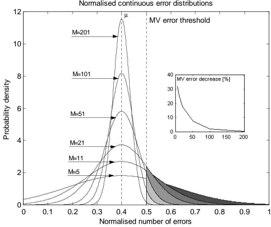
FIGURE 3. A family of normalised continuous error distributions for increasing number of classifiers with the same individual errors of 40%. Decreasing shaded area corresponds to reducing majority vote error. The relation between this error reduction and the number of independent classifiers is shown in the subfigure.
