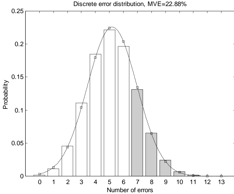
FIGURE 1. Discrete error distribution with normal distribution approximation. Parameters: 13 independent classifiers with 40% error each. Shaded bars refer to errors in majority voting sense. The MV error rate corresponds to the sum of all shaded bars.
