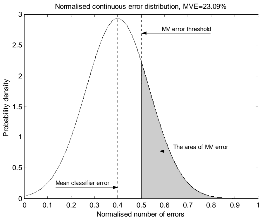
FIGURE 2. Normalised continuous error distribution. Parameters: 13 independent classifiers with 40% error each. Shaded area refers to majority voting error rate.
