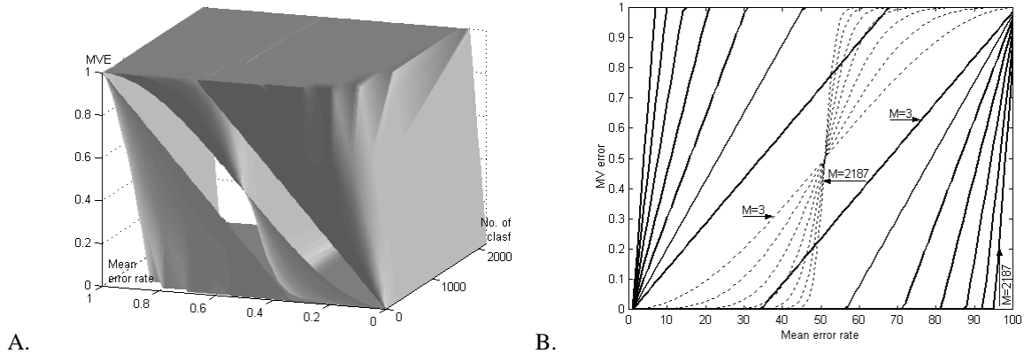
FIGURE 12. The error limits of MOMV shown as a function of the number of classifiers and the mean classifier error. A. 3D plot including surface corresponding to MOMV errors for independent classifiers. B. 2D projections for the selected numbers of classifiers.
