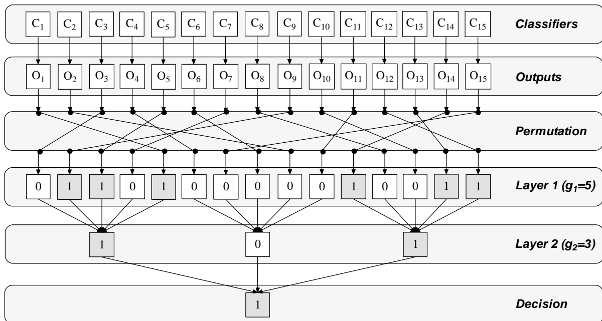
FIGURE 10. The scheme of the multistage organisation system with 15 classifiers, structure S_{15} = (5,3) and permutation P_{15} = (3,9,5,7,1,4,15,6,2,11,14,8,10,13,12) . Trained classifiers C_1, \dots, C_{15} produce binary outputs O_1, \dots, O_{15} (1-correct, 0-incorrect), which after permutation P_{15} are subsequently grouped and aggregated by majority voting at each layer according to the structure S_{15} . The final output is reached at the decision layer.
