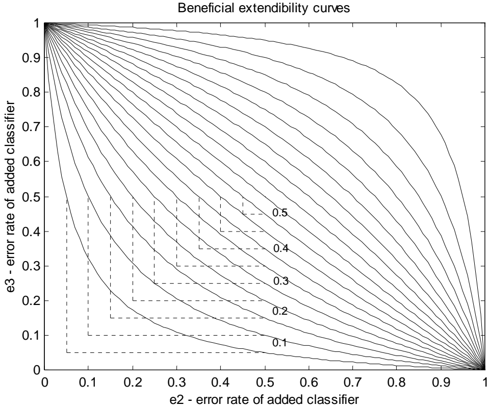
FIGURE 5. Extendibility curves for different errors of a single classifier. Dashed lines limit the area corresponding to individual errors of joining classifiers e_2, e_3 greater than error e_1 but producing MV error lower than e_1 .
