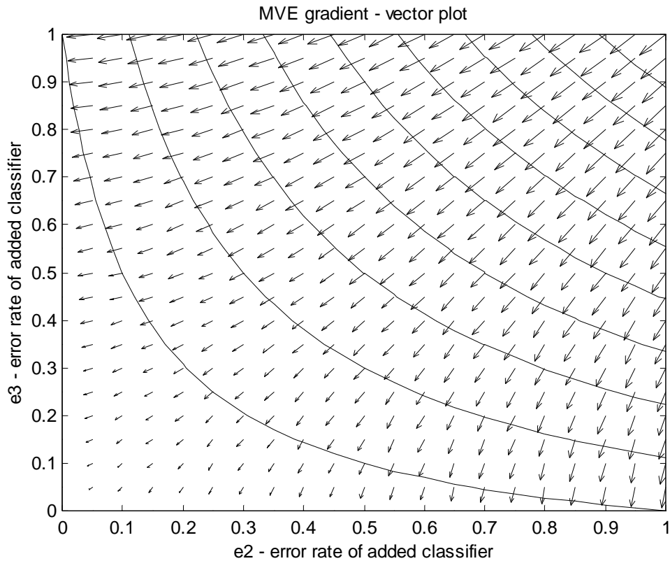
FIGURE 4. Majority voting error as a function of individual errors of a joining pair of independent classifiers e_2, e_3 . Parameters: MCS with 1 classifier at error level e_1 = 10\% . Solid lines correspond to the same combined MV error out of all 3 classifiers. The vectors visualising gradient of the combined error, point in the directions of the maximal reduction of MV error.
