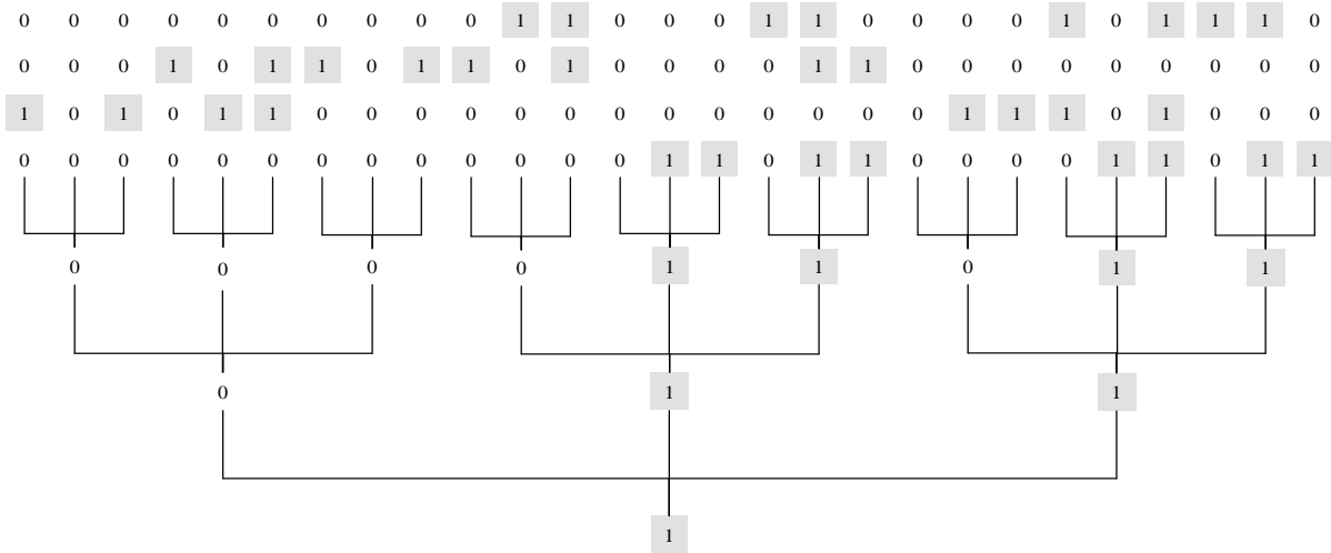
FIGURE 11. Optimal multistage organisation with 27 classifiers structured by optimal structure: S_{27} = (3,3,3) . Optimality of error distribution enforces the presence of exactly 8 correct votes for every data sample. Examples of optimal permutations are shown above the structure.
